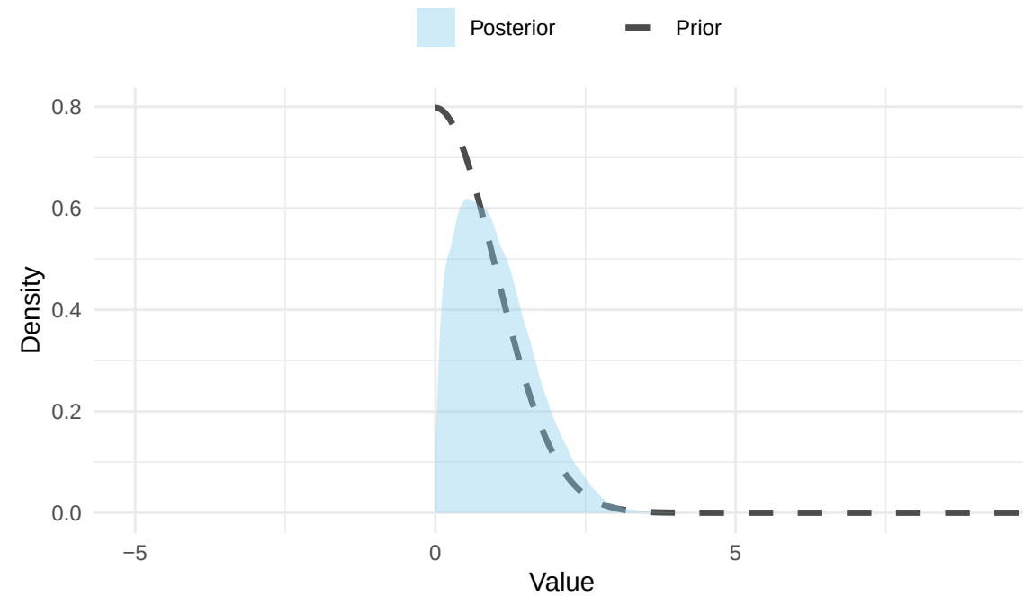
Prior vs Posterior: sigma
